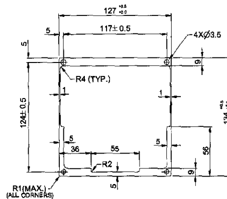
VIEW FROM - F (KEY PAD SEAT PROFILE)
