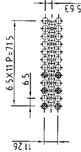
DETAIL - 'A'
